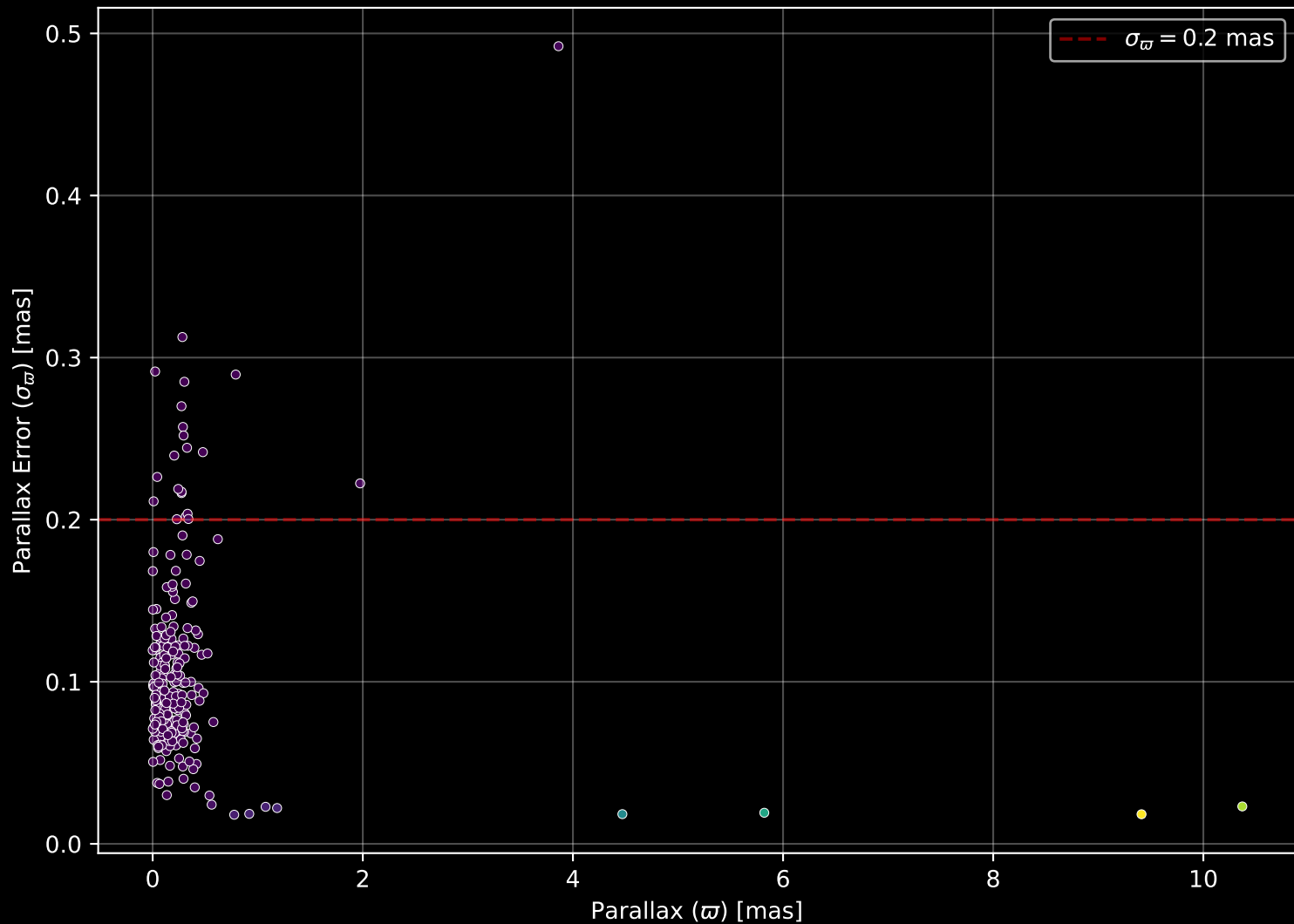
APOGEE DR17 Field: [000+04-O] Parallax Quality (n= 246)
