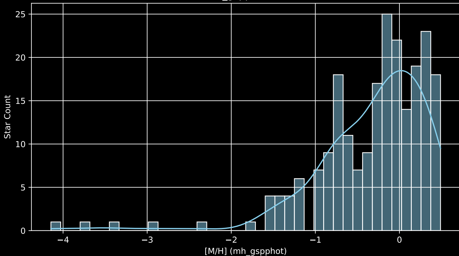
APOGEE DR17 Field: [000+04-O [M/H] (mh_gspphot) (n= 223)
