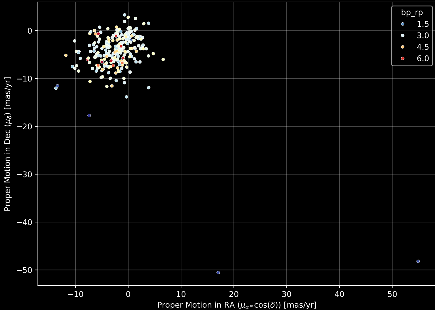
APOGEE DR17 Field: [000+04-O] Proper Motion Diagram (n= 246)
