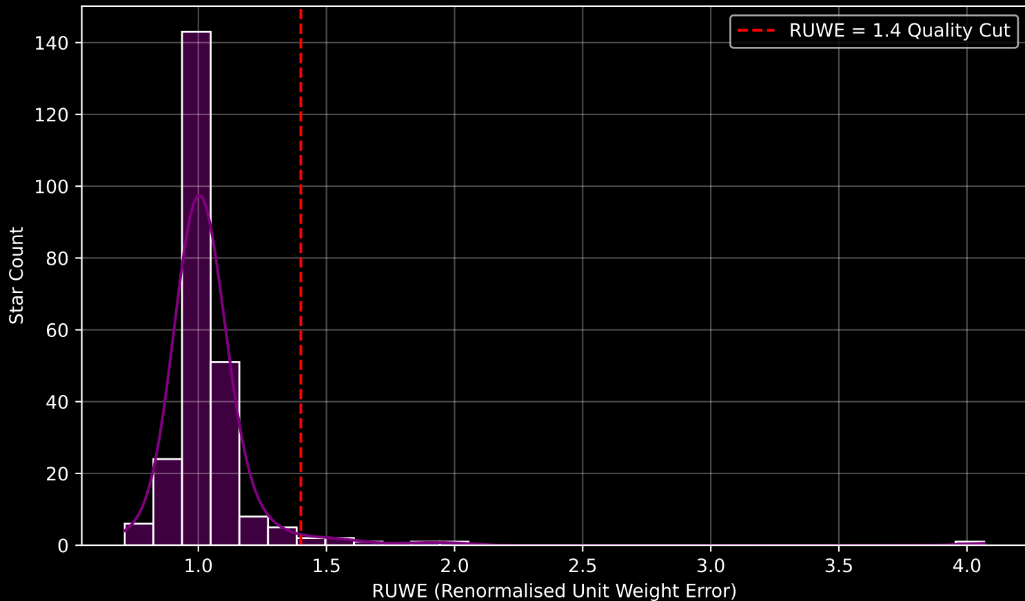
GAPOGEE DR17 Field [000+04-O] RUWE Distribution (n= 245)
