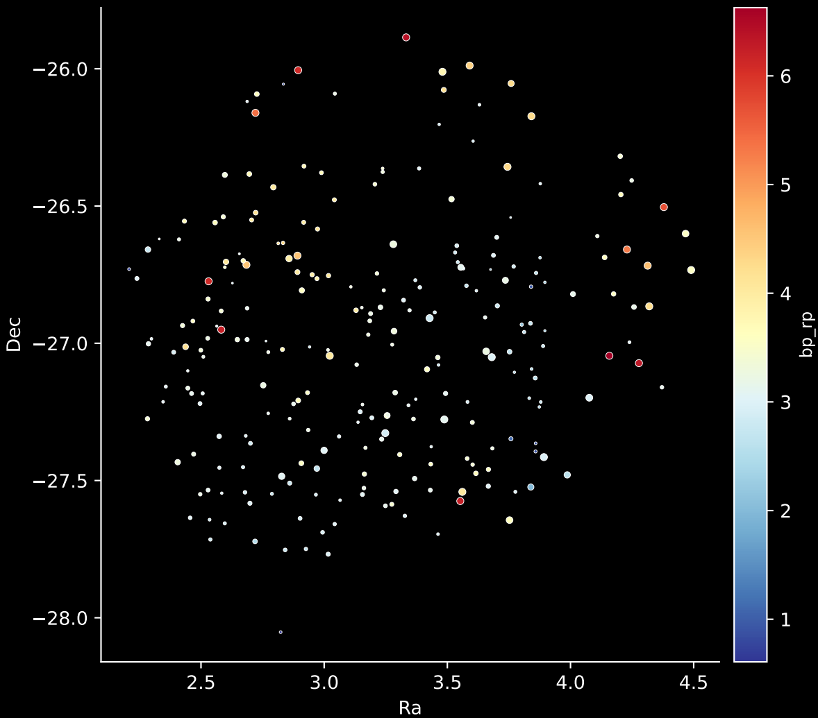
APOGEE DR17 Field: [000+04-O] Stars: 246
